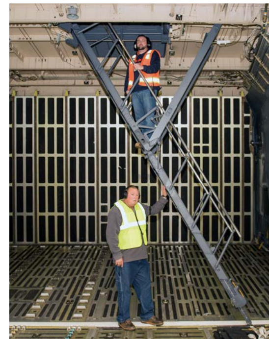
Interior Ladder of C-5, 14 Steps
