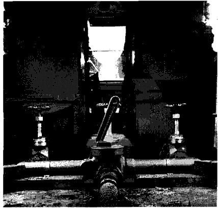
The cabins of the receiver (left) and the tanker. In the receiver, the fueling hose was placed in the funnel, which fed the cabin tanks under the duck boards at center. The tanker's refueling system has three gate valves, a levered quick closing valve, and a strainer in front of the hose.
