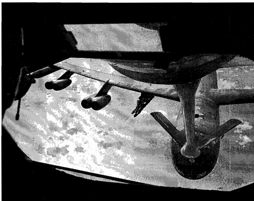
View over the right shoulder of a KC-135 boom operator as a B-52 armed with bombs for a mission over Vietnam approaches for refueling. The B-52's open refueling receptacle can be seen just to the right of the boom.
