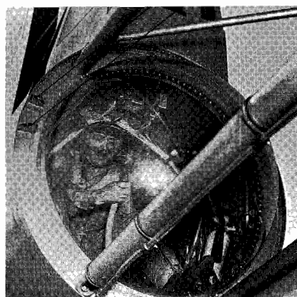
The earliest model of the Boeing boom was temporary, with exposed girders, cables, and pulleys. The boom operator in the KB-29P sat in what had been the tailgunner's space.
