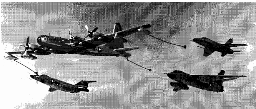
A TAC KB-50 trails three drogues for refueling. An RF-101 is connected (left), while a B-66 (center) and a F-100 (right) move up to connect.
